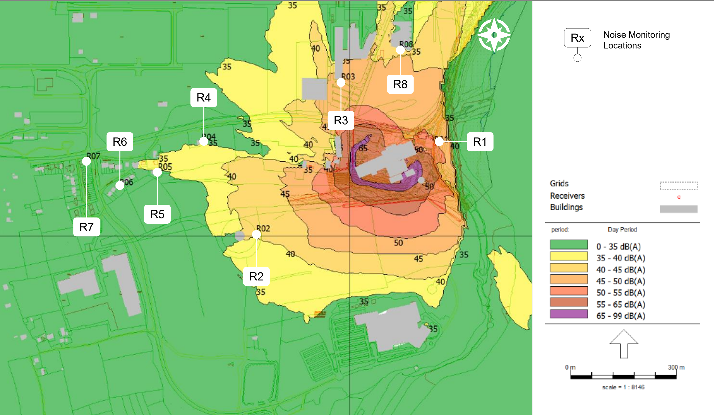
Figure Title: Operational Modelled Scenario 1 – Calculated Noise Contours Figure No. 10.9
